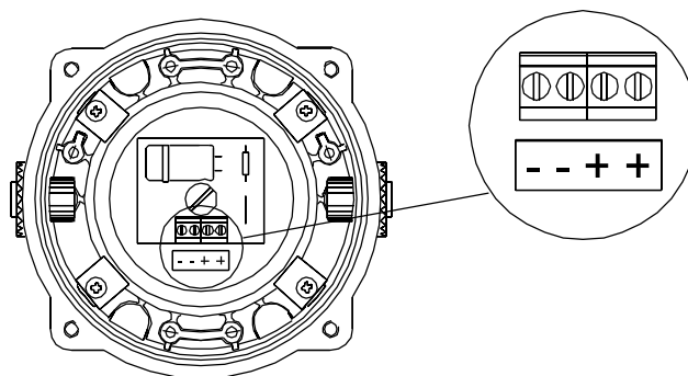
BExL25D & BExL15D 8 ohm and 16 ohm
