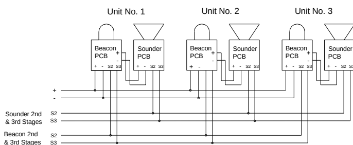
BExDCS110-L1D DC Combined Sounder Unit LED Beacon and Sounder Wired for Simultaneous Operation
