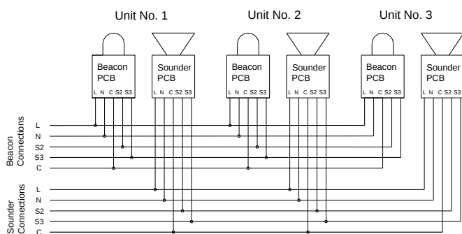
BExDCS110-L1D AC Combined Sounder Unit LED Beacon and Sounder Wired for Independent Operation
