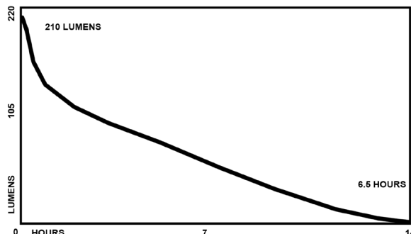
XPP-5422GX PERFORMANCE CURVE
