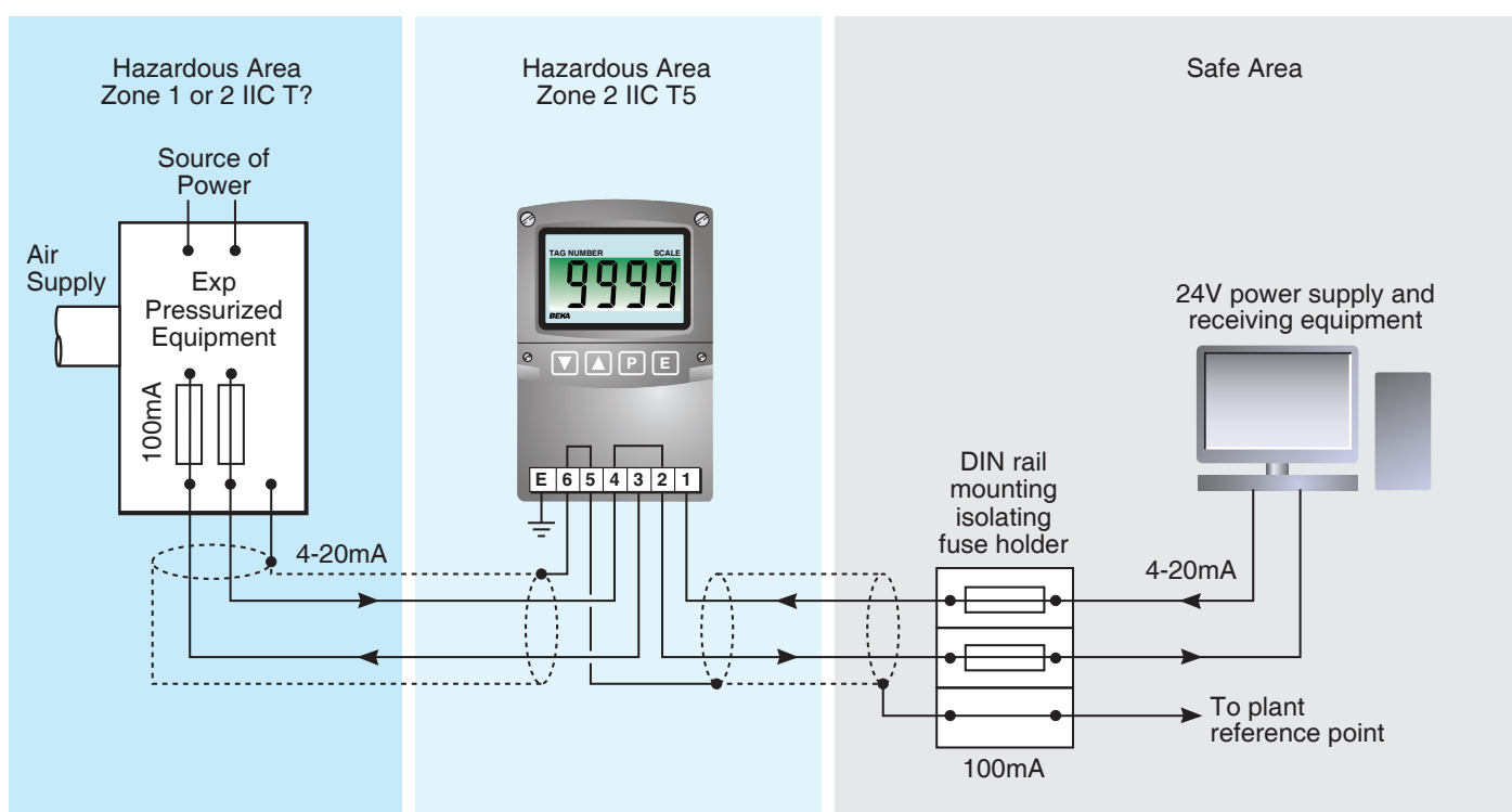
Figure 14. Indicator in Zone 2 monitoring signal from powered pressurized equipment with a source of power
