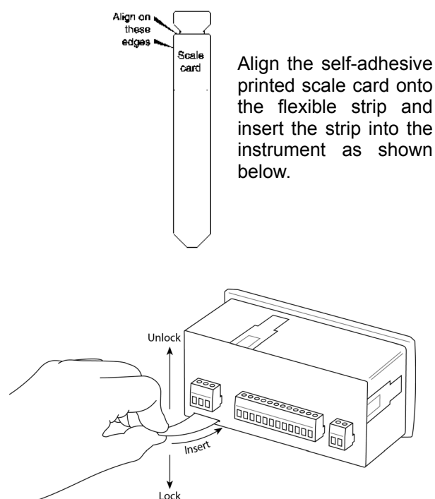
Fig 13 Inserting the flexible strip carrying the scale card into slot at the rear of the instrument.
