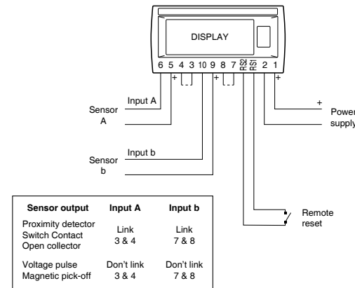
Fig 3 Typical system
