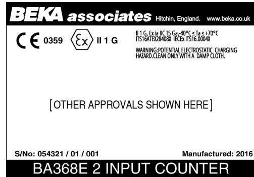
BA368E Certification information label
