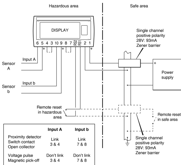
Fig 2 BA368E used with Zener barriers
