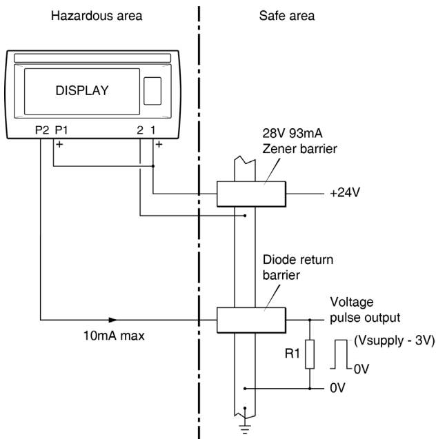
Fig 12 Generating voltage pulse in safe area using Zener barriers.
