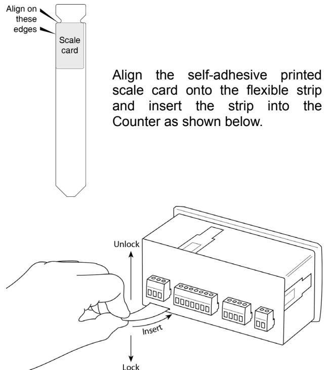
Fig 8 Inserting the flexible strip carrying the scale card into slot at the rear of the BA368E Counter.
