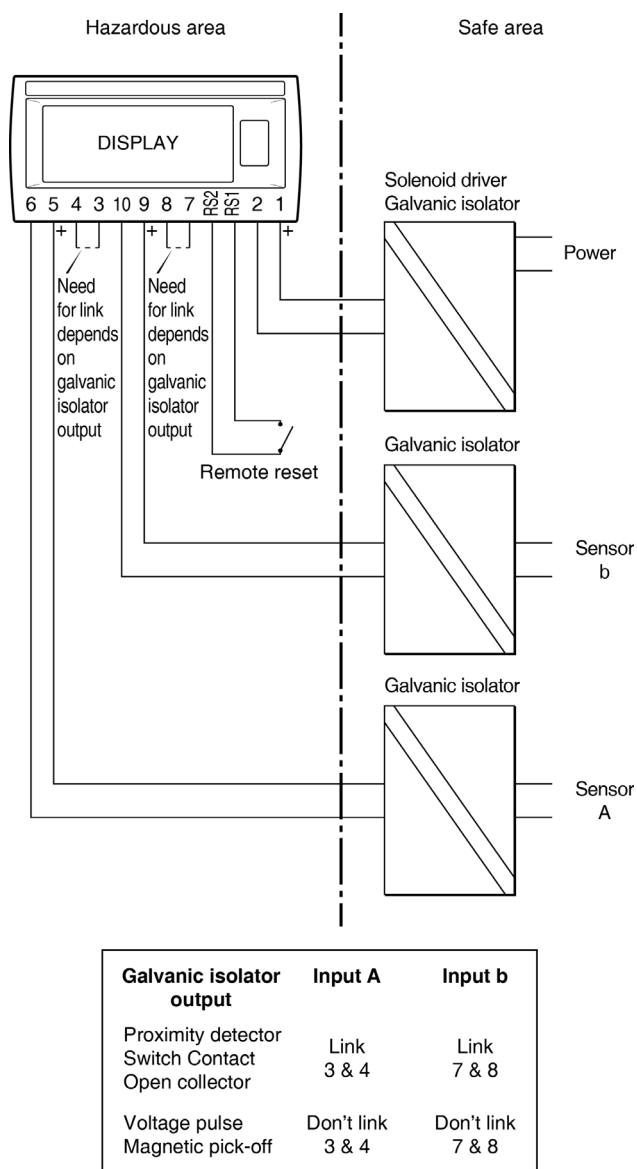
Fig 5 Pulse source in safe area
