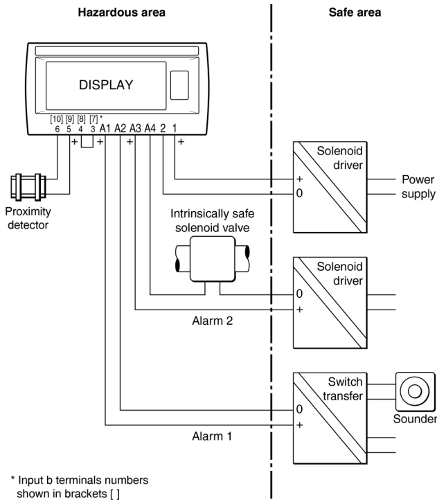
Fig 15 Typical alarm application
