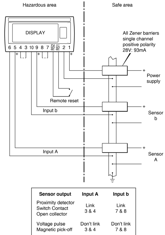
Fig 3 BA368E used with Zener barriers pulse source in safe area.
