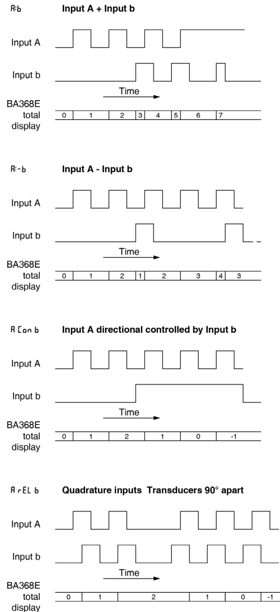
Fig 11 Counting waveforms
