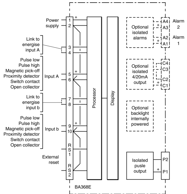
Fig 1 BA368E block diagram
