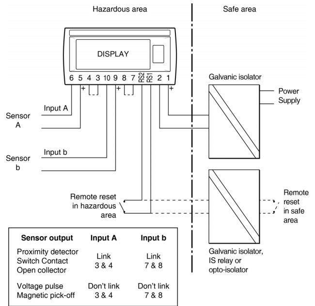
Fig 4 BA368E protected by galvanic isolators.
