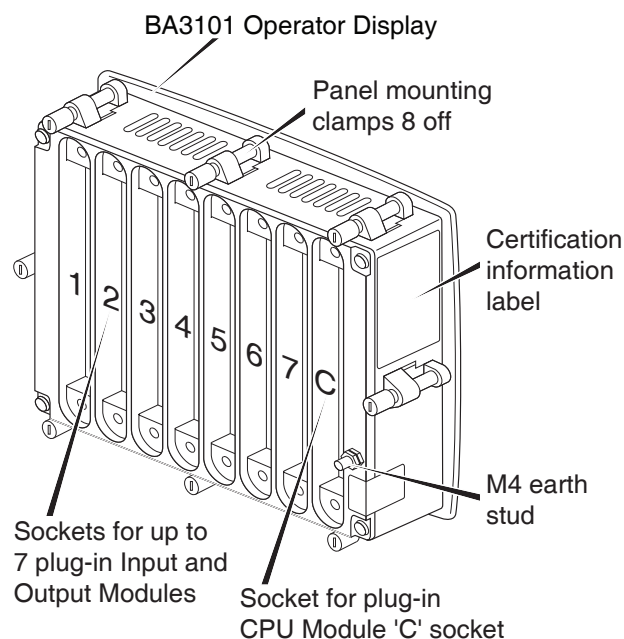
Fig 1 Rear view without plug-in modules
